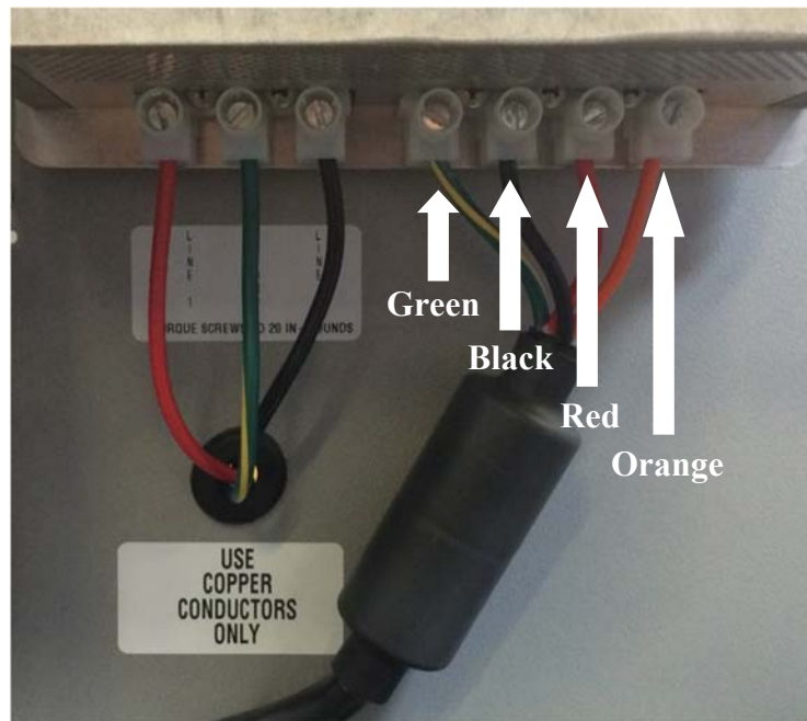
Figure 15 – Cord Reel Wiring Termination
