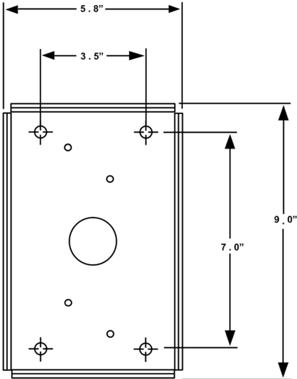
Figure 1 – L2 PowerPost® EVSE Footprint & Mounting Hole Locations
