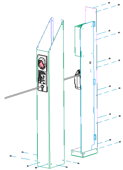
Figure 5 – Front Housing Removed
