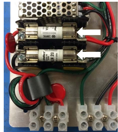
Figure 14 – Power Fuse
