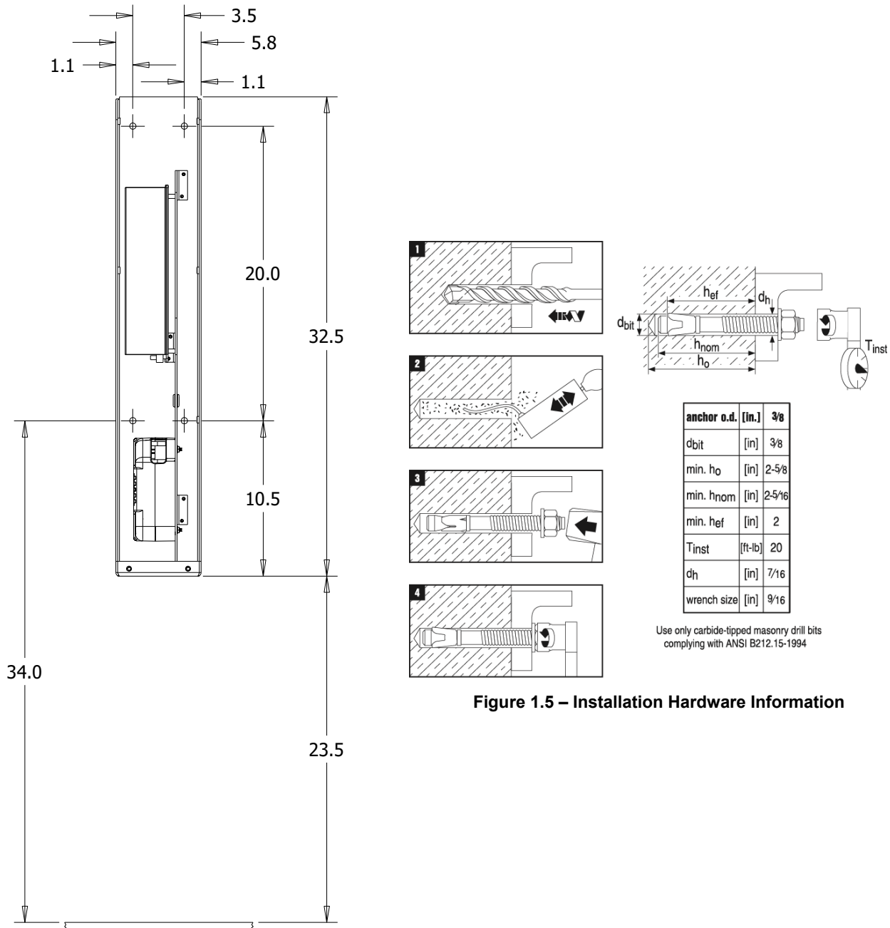
Figure 1 – L2 PowerPost® EVSE Mounting Hole Locations
