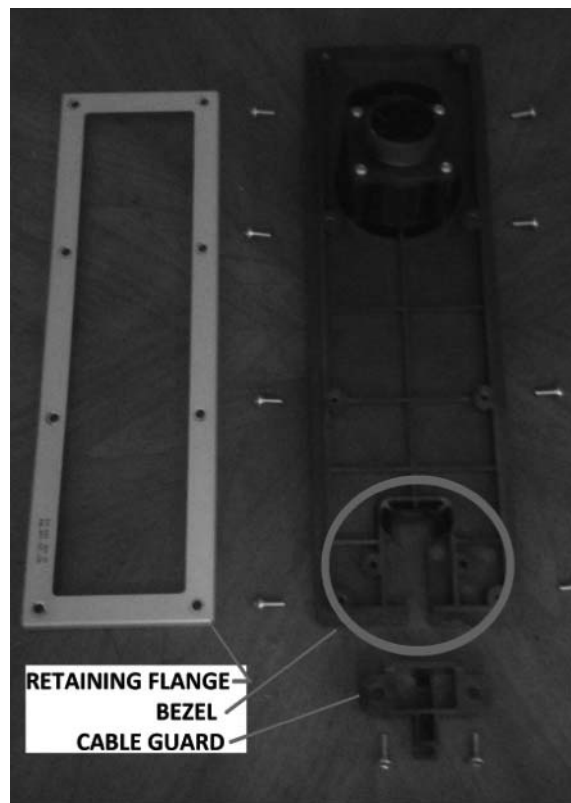
Figure 17 – Front Bezel Disassembled
